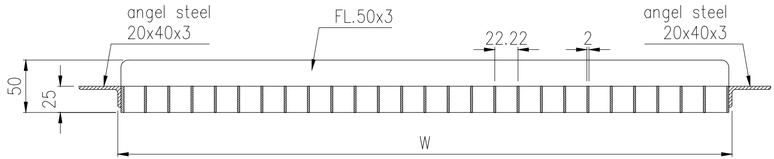
Section B-B
