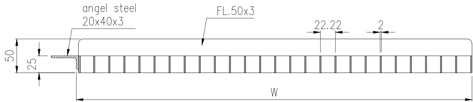
Section B-B
