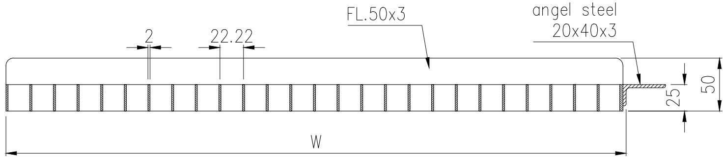
Section B-B
